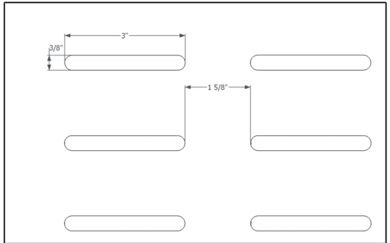
3 Slot Pattern Perforation: 3" x 3/8" Spacing: 2" OC
