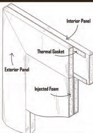
First Generation Thermal Break
