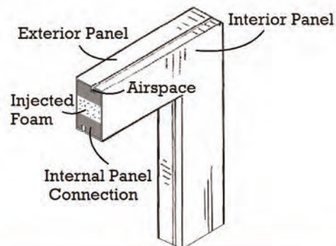
Second Generation Thermal Break
