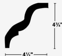
224 - Design Cornice
