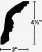
188 - Design Cornice
