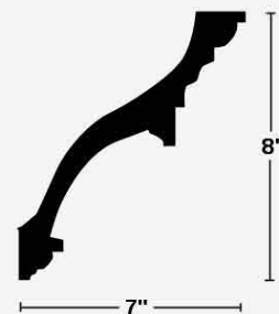
247 - Design Cornice
