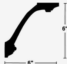
163 - Design Cornice
