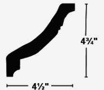
208 - Design Cornice
