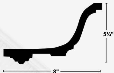
218 - Design Cornice
