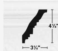
173 - Design Cornice
