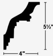
172 - Design Cornice
