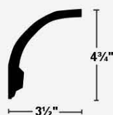
244 - Design Cornice
