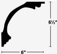
261 - Design Cornice
