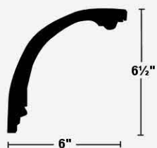
156 - Design Cornice
