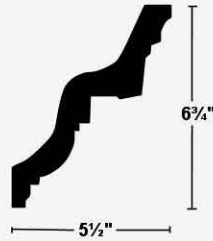
148 - Design Cornice
