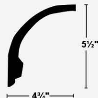
226 - Design Cornice
