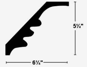
262 - Design Cornice Available in smaller size
