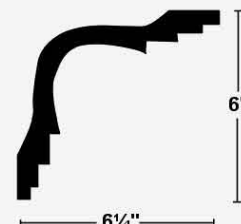
249 - Design Cornice
