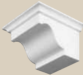
BL 2509 • 9 7/8" Projection • 5 3/4" Height • 8 5/8" Width
