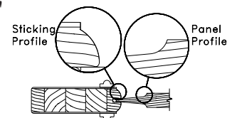
"STANDARD HIP" PROFILE
