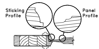
"DOUBLE HIP" PROFILE
