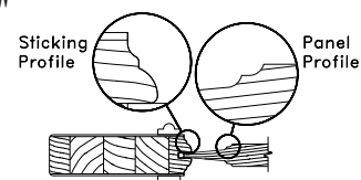
"COVE & BEAD" PROFILE
